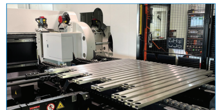
3-D pipe laser processing machine (FABRI GEAR 400 III (MAZAK)) at Osaka factory
