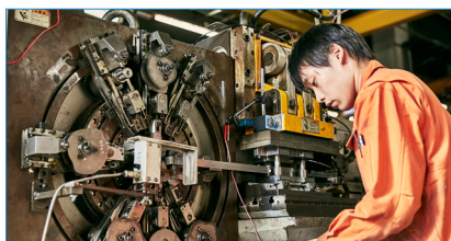
Multi forming machine at flat spring factory
