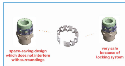
Lock mechanism of "CROWN"
